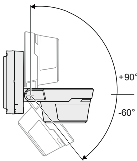
Fig. 23: Transmission range
